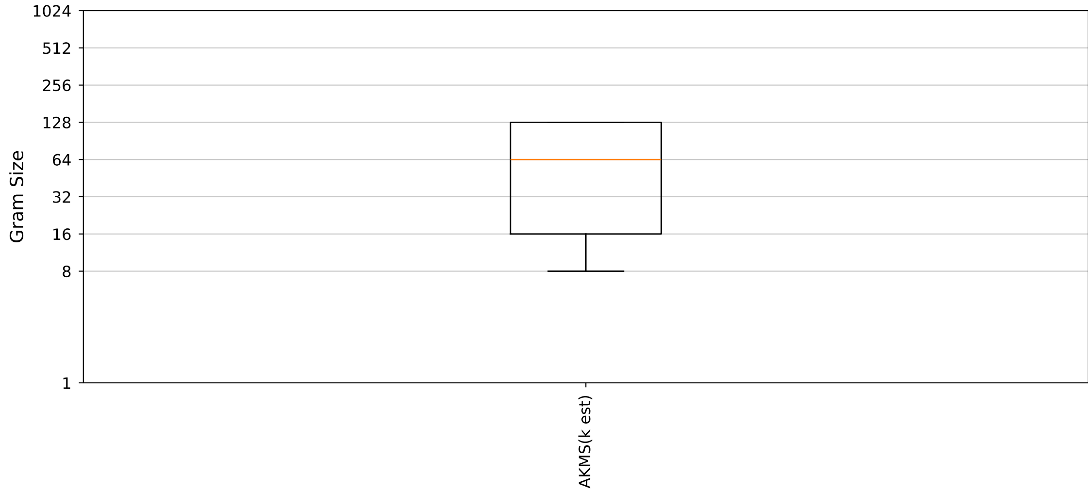
YARA Rules Gram Size Distribution (Cluster3_Size53 dataset)
